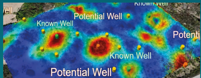
3D rendering of the inspected site with a photogrammetry layer
